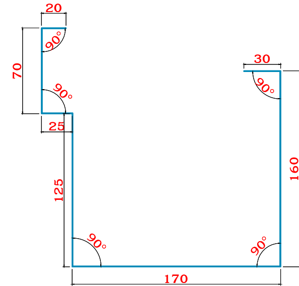
EAVE GUTTER 0.5 mm Thick
