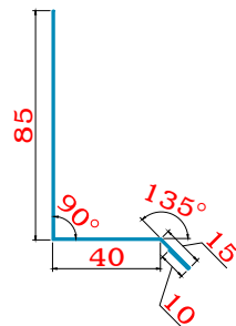
DRIP TRIM 0.5 mm Thick
