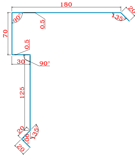
GABLE TRIM 0.5 mm Thick
